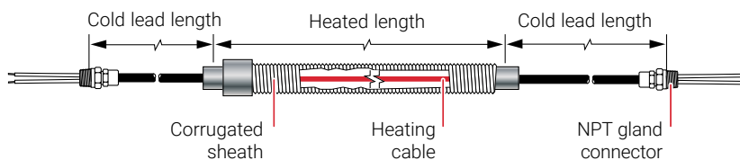
Dual conductor cable (XMI-L32 or XMI-L62 series)
