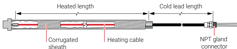
Dual conductor cable (XMI-L32 or XMI-L62 series)
